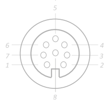
M12 8-Pin Connector A-Coding Male*
