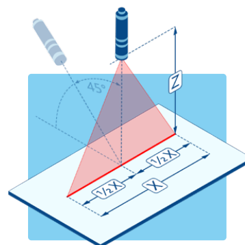
(b) Vertical installation (up to 45°)
