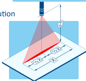
(b) Vertical installation (perpendicular 90°)
