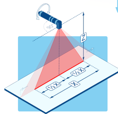
(c) Beam perpendicular to the housing (tiltable)
